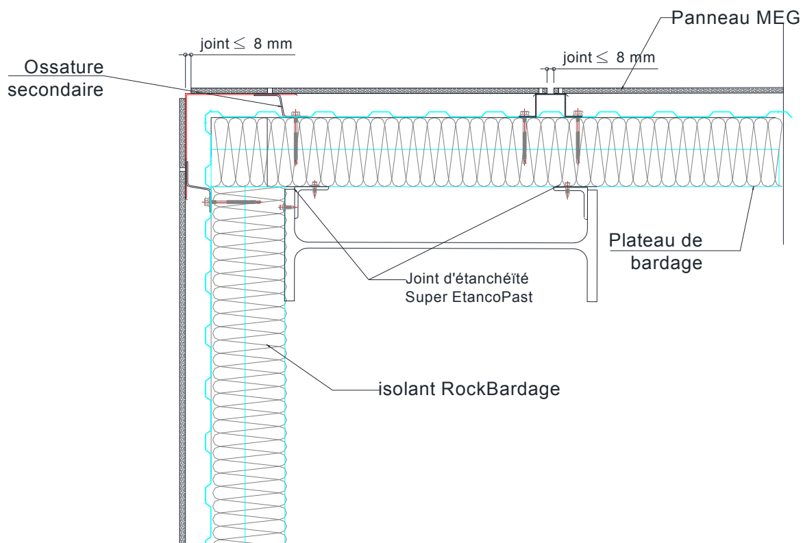
Figure 18 – Angle sortant
