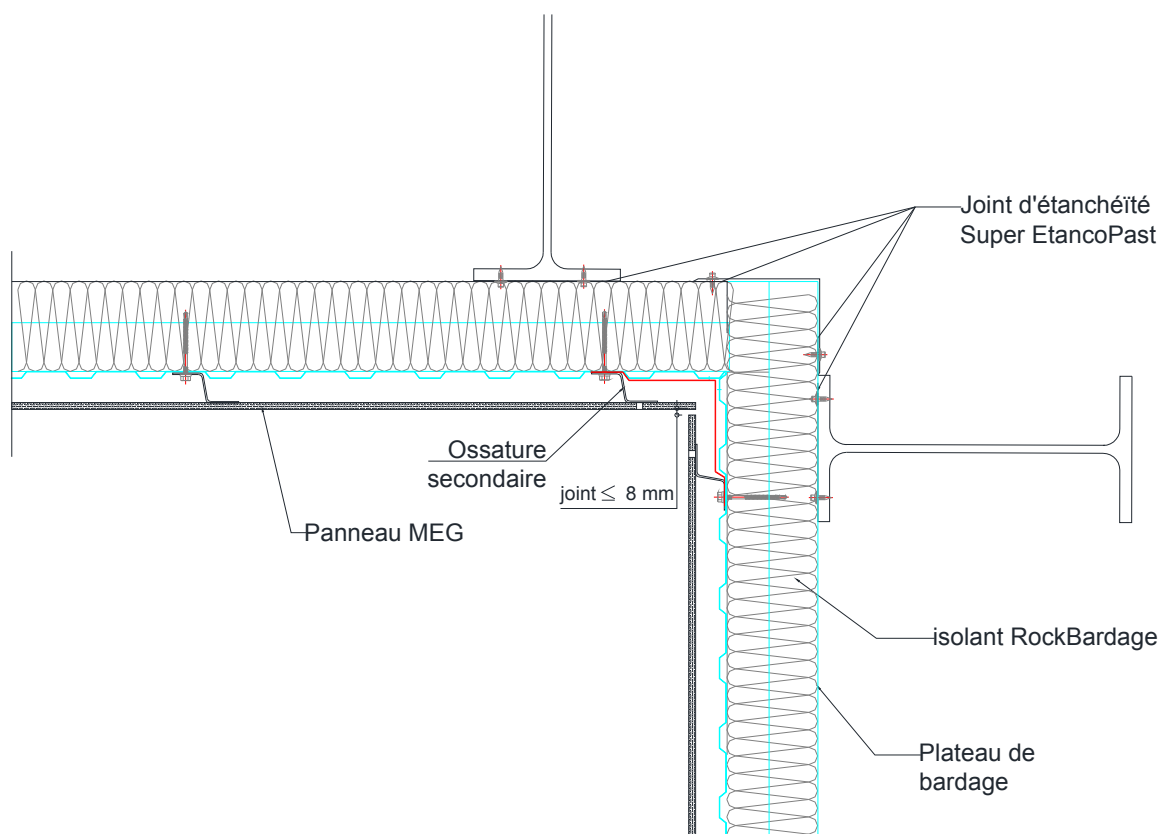
Figure 19 – Angle rentrant
